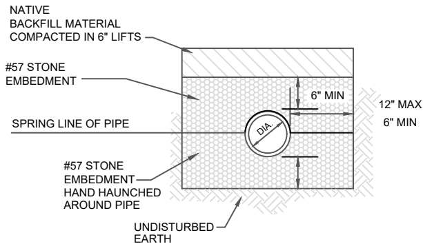
STANDARD EXCAVATION
