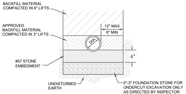
UNDERCUT EXCAVATION IN UNSTABLE SOILS TYPES
